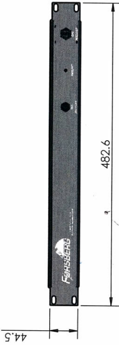
FRONT ELEVATION SCALE 1:4
