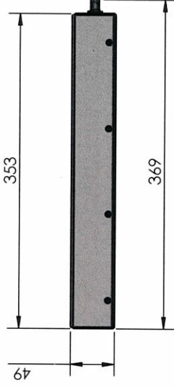
SIDE ELEVATION SCALE 1:4
